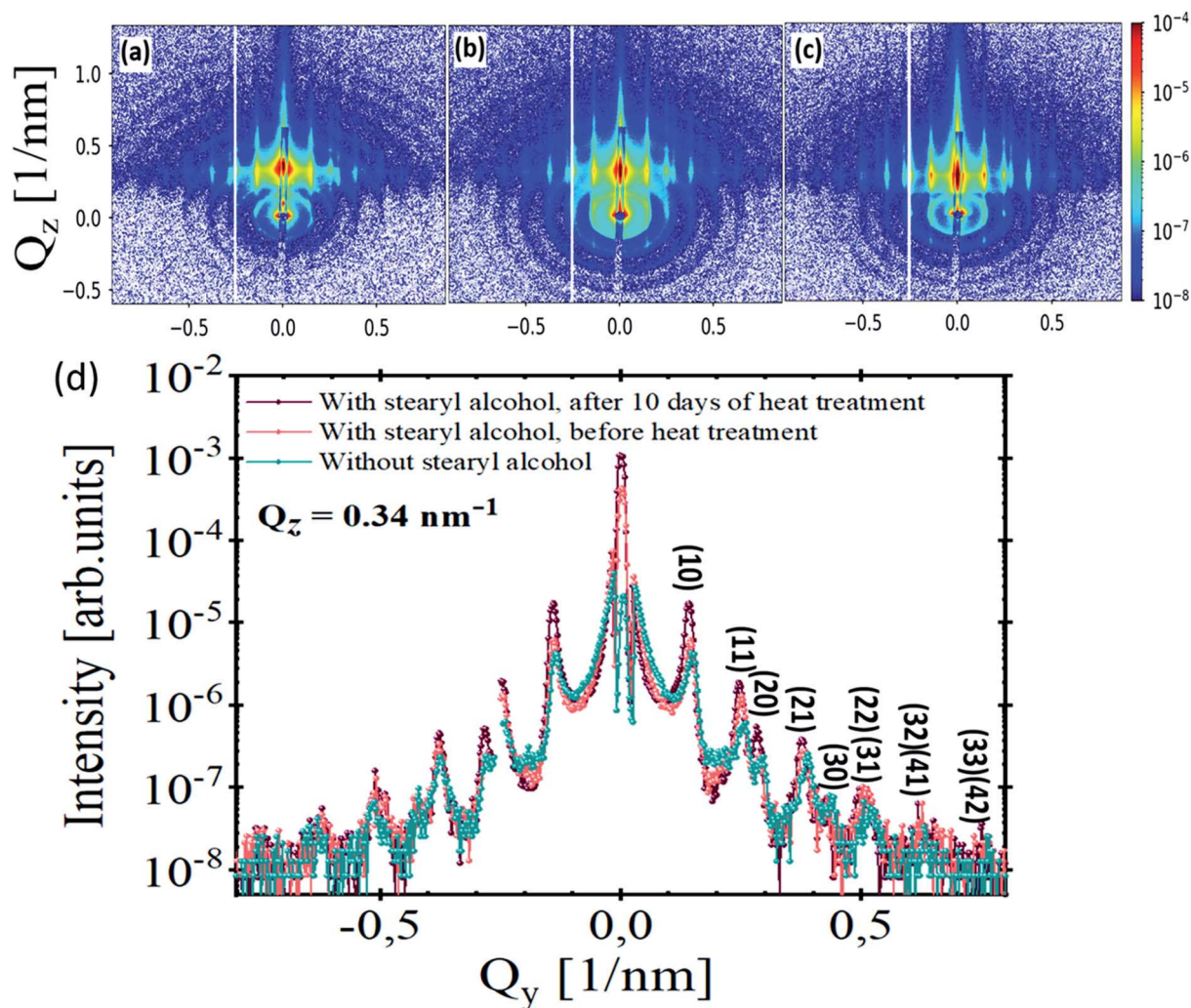
Fig. 6 GISAXS pattern of a monolayer of SiO 2 NPs deposited on silicon substrates (a) before using stearyl alcohol (b) after using stearyl alcohol, before heat treatment and (c) after 10 days heat treatment. (d) Line-cuts from (a), (b) and (c) along Q_y at a constant Q_z = 0.34 \text{ nm}^{-1} . The Bragg peaks are indexed by assuming a 2-D hexagonal lattice with a lattice constant a = 51.6 \pm 0.4 \text{ nm} .
